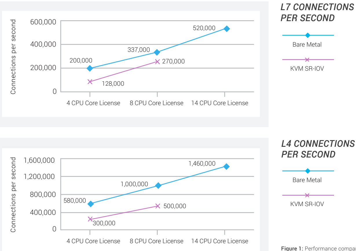
Figure 1: Performance comparison between bare metal and KVM SR-IOV.1
