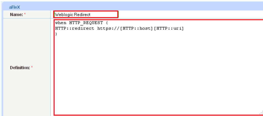
Figure 34: Redirect script
