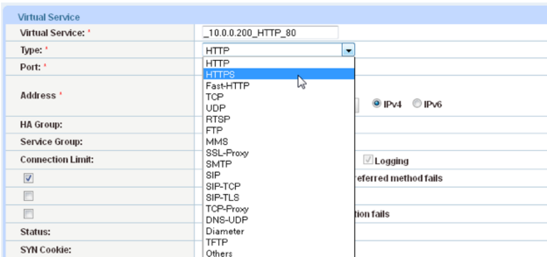
Figure 17: Virtual service configuration
