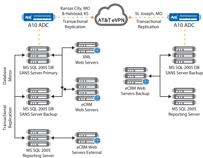
Figure 1: USA 800 database and web server architecture
